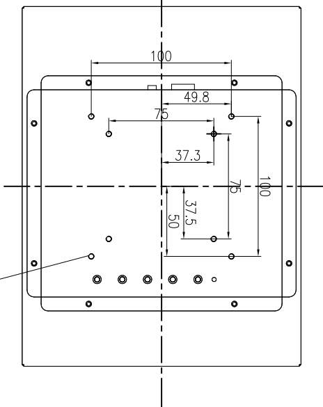
Back View
