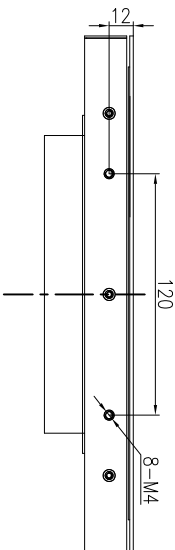
Bottom View
